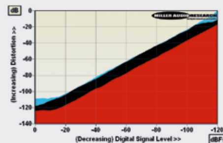
ABOVE: Distortion vs. digital signal level over a 120dB range (1kHz/24-bit, red; 1kHz/CD, black; 20kHz, blue)
