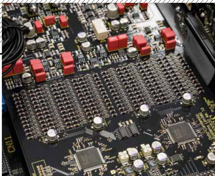
LEFT: The 96 latches (a matrix of 2x48) that comprise the Rossini's Ring DAC core are clearly visible here, driven via two Xilinx Spartan DSPs sitting alongside [see also boxout, below]
