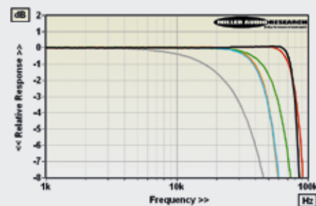
ABOVE: Frequency responses with 192kHz data (Filter 1, black; 2, red; 3, cyan; 4, green; 5, grey; Filter 6, orange)
