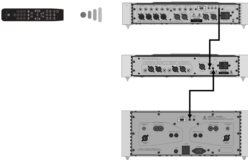
Figure 8: Remote operation with 12V trigger
