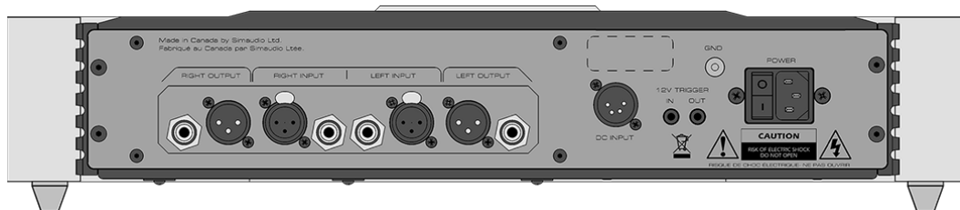
Figure 6: 610LP Rear panel
